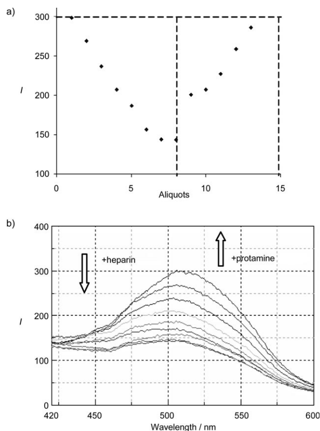
Figure 4. Reverting heparin binding by 6 upon titration with protamine. a) Addition of eight aliquots of heparin to polymer 6 (33 nM), followed by five aliquots of protamine: the fluorescence emission is fully restored. b) Fluorescence emission quenching of 6 upon addition of increasing amounts of heparin (30–220 nM). Subsequent protamine addition restores the original emission intensity.
