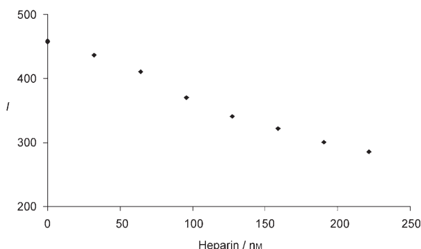
Figure 5. Calibration curve displaying a linear correlation between fluorescence emission intensity and heparin concentration from 30 nm to 0.22 \mu\text{M} heparin (25 mM HEPES buffer).
