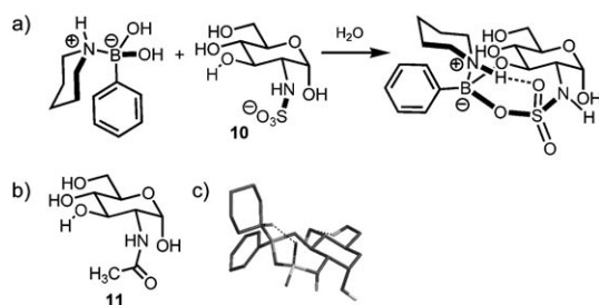
Figure 3. a) Model complexation mixture, consisting of D-glucosamine 2-sulfate sodium salt ( 10 ) and the preformed 1:1 aggregate from phenylboronic acid and piperidine. b) Reference compound 11 . c) Proposed structure of the preferred complex. Note that the boronic acid moiety forms a seven-membered ring with the 3-OH group and the 2-aminosulfate.
