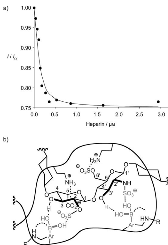
Figure 2. a) Fluorescence quenching by addition of heparin (LMWH) to polymer 6 in 25 mM HEPES buffer. The K_a value obtained from this curve was calculated at 2.8 \times 10^7 \text{ M}^{-1} (stoichiometry HEP/6 6:1). b) Proposed wrapping mechanism with favorable interactions between polymer and heparin. The B...N interaction was not specified, it is most likely a hydrated species. [15]
