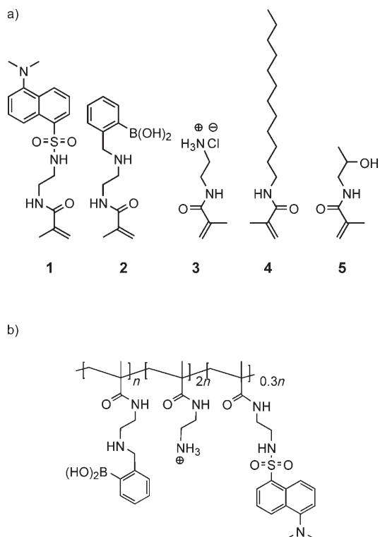
Figure 1. a) Functional comonomer structures. 1 : dansyl, 2 : boronic acid, 3 : ammonium, 4 : dodecyl, 5 : amino-alcohol unit. b) Schematic representation of a selected copolymer ( 6 ).
